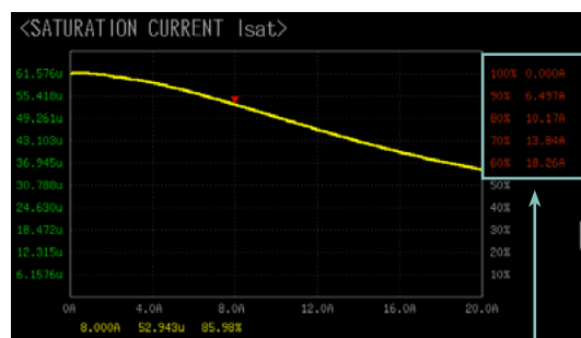
Inductance Decrease Percentage (%)
